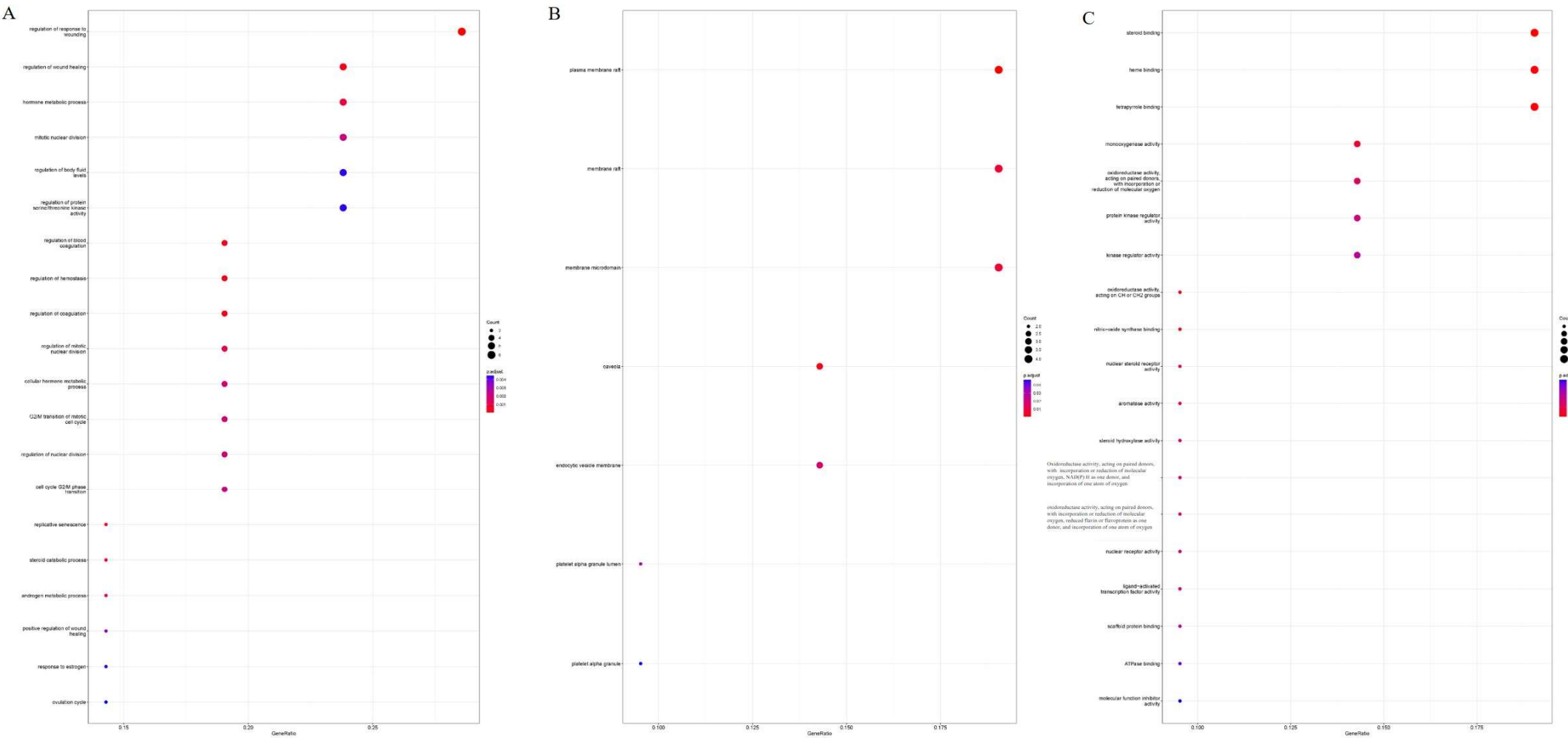
Supplementary Figure A Enrichment analysis of shared targets in Gene Ontology terms. (A) BP, (B) CC and (C) MF. BP, biological process; MF, molecular function; CC, cellular component
